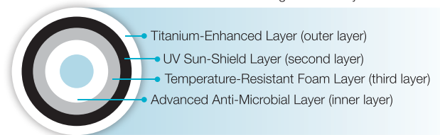
Cross-section of 'Ganga Cool 4 Layer' water tank
