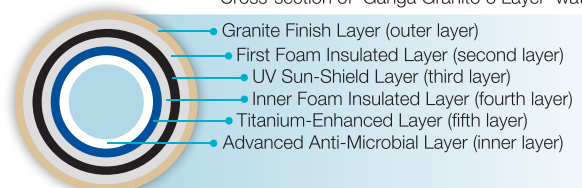
Cross-section of 'Ganga Granito 6 Layer' water tank
