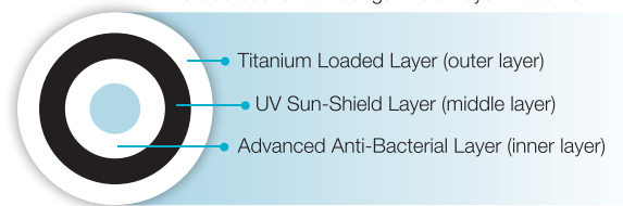
Cross-section of 'Ganga Pro 3 Layer' water tank
