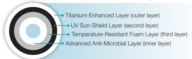
Cross-section of 'Waterwell Italian 4 Layer' water tank
