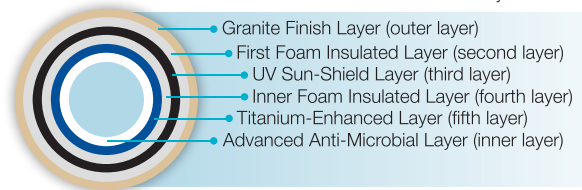
Cross-section of 'Waterwell Granito 6 Layer' water tank
